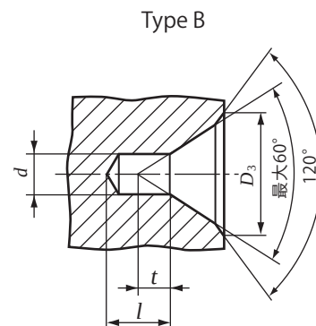
Form with chamfering (Drilling centre bore from JIS B4304)
