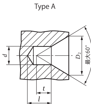
Form without chamfering (Drilling centre bore from JIS B4304)
